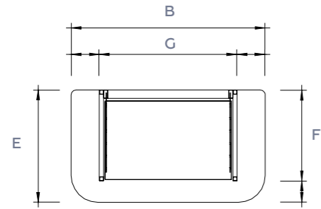
1: Plan
