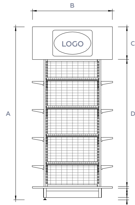
2: Side Elevation
