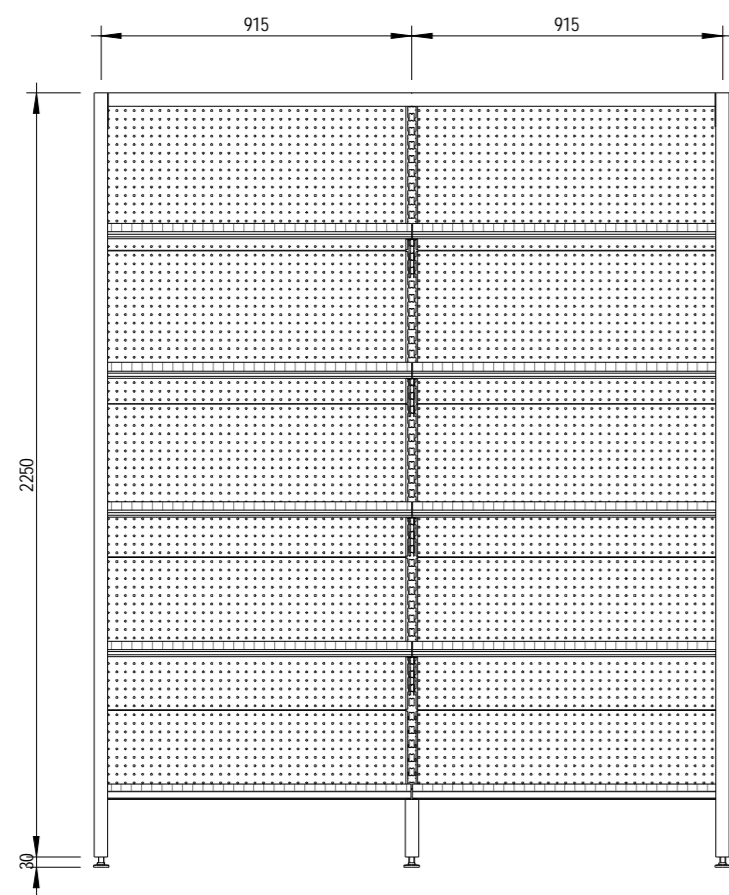
2 Side Elevation 1 : 20
