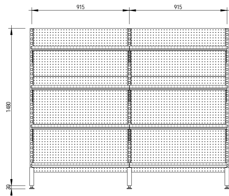
2 Side Elevation 1 : 20
