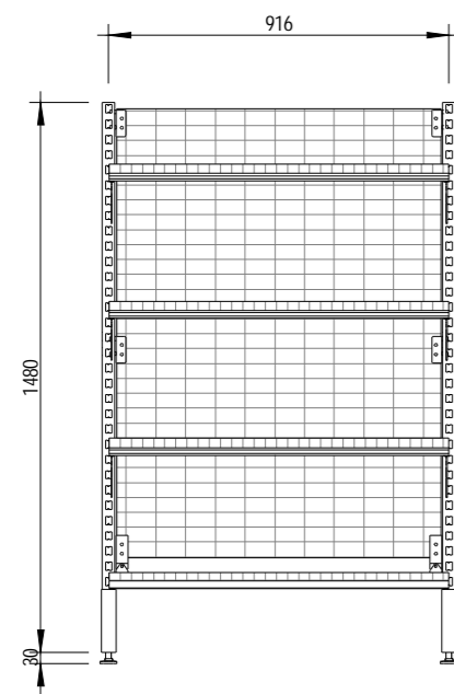
2 Side Elevation 1 : 20
