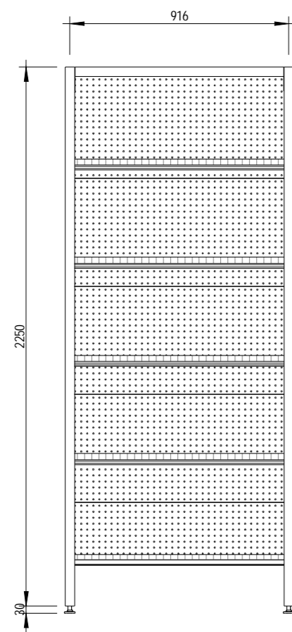
2 Side Elevation 1 : 20
