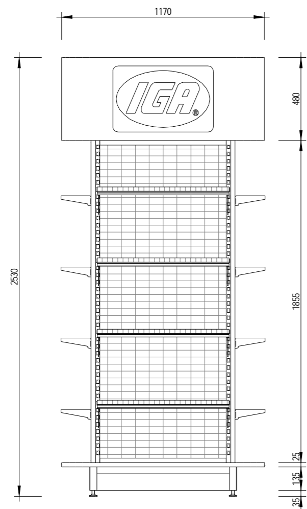
2 Side Elevation 1 : 20
