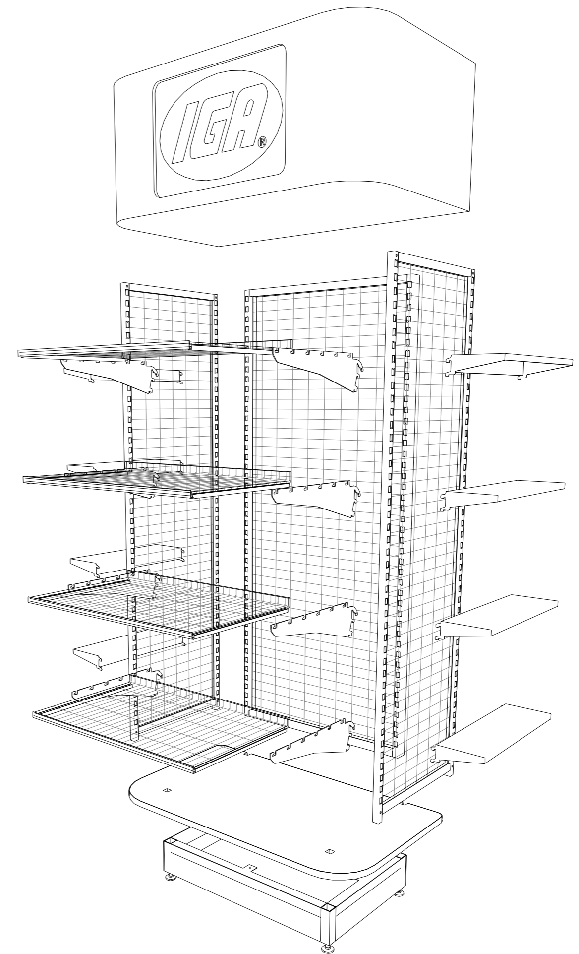
4 3D Assembly
